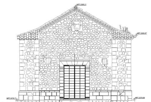
Fachada Principal
